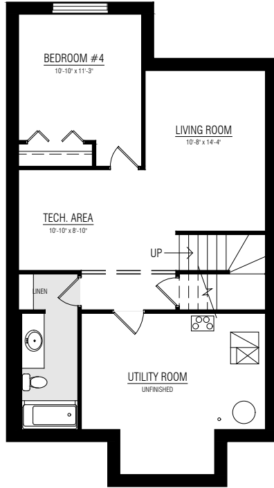
BASEMENT DEVELOPMENT 588 SQ. FT.
