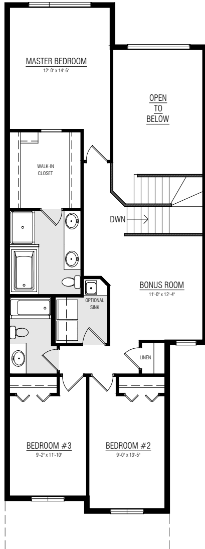
UPPER FLOOR STANDARD 1112 SQ. FT.
